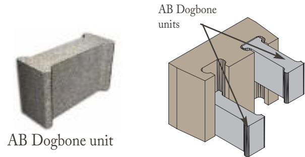
Parapet graphics are to show facing unit and AB Dogbone unit placements. All parapet installations need to include wall rock in cores.
